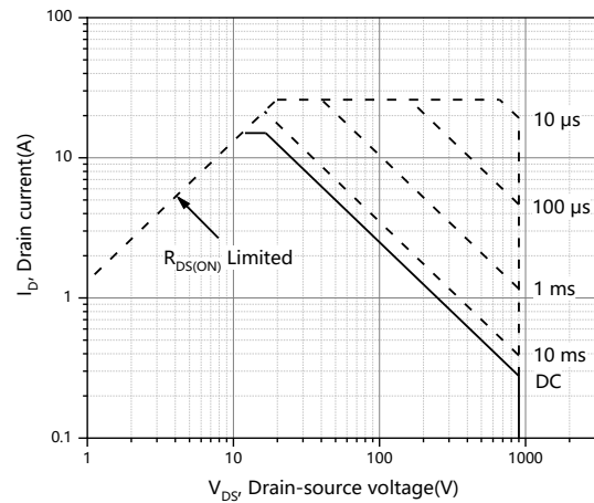
Figure 12. Safe operation area for T_C = 25 \text{ °C}
