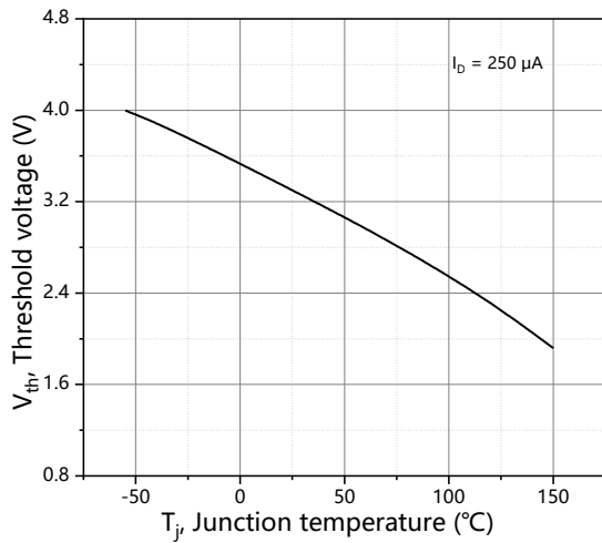
Figure 7. Threshold voltage
