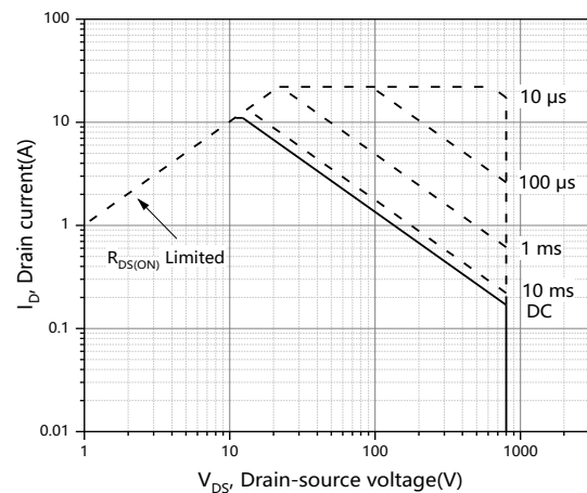
Figure 12. Safe operation area T_C=25^\circ C
