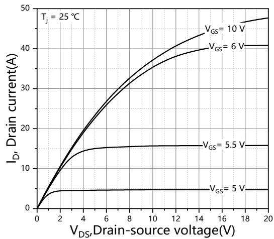
Figure 1. Typ. output characteristics T_j=25\text{ °C}
