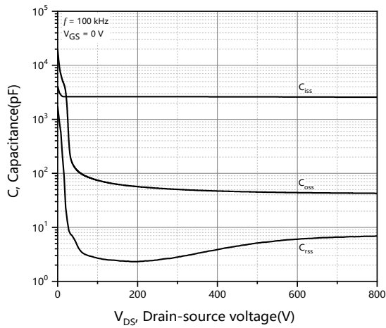
Figure 3. Typ. capacitances
