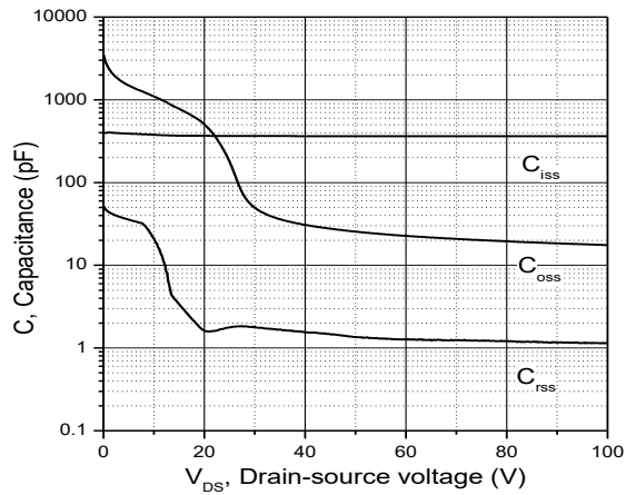
Figure 3. Typ. capacitances
