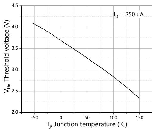
Figure 7. Threshold voltage
