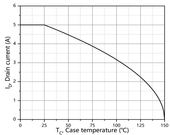
Figure 10. Drain current
