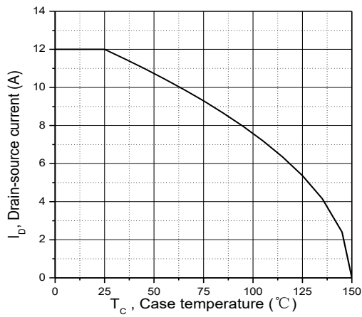
Figure 9. Drain current
