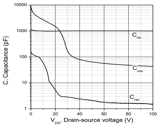
Figure 3. Typ. capacitances
