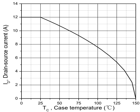
Figure 9. Drain current
