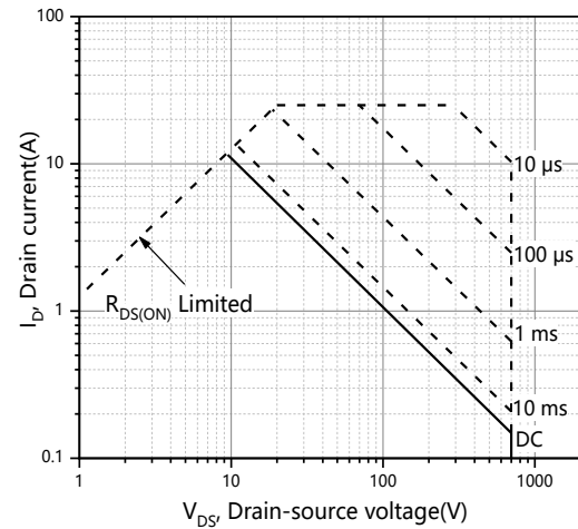
Figure 12. Safe operation area for Tc=25°C
