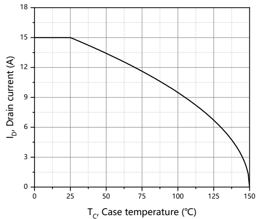
Figure 10. Drain current
