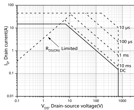
Figure 12. Safe operation area T_c=25^\circ C
