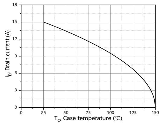
Figure 10. Drain current
