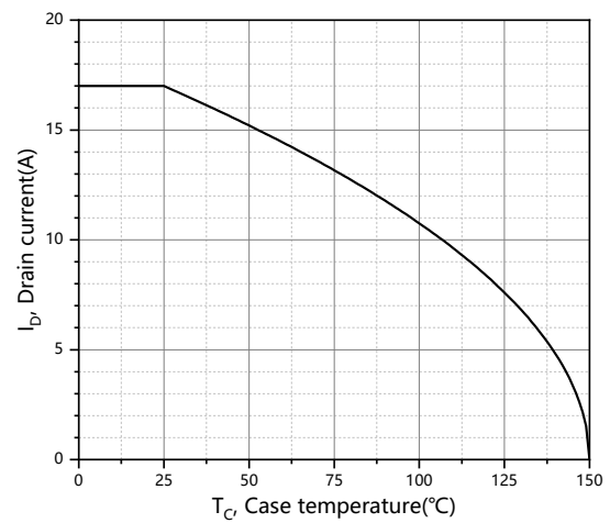
Figure 10. Drain current
