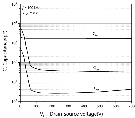
Figure 3. Typ. capacitances
