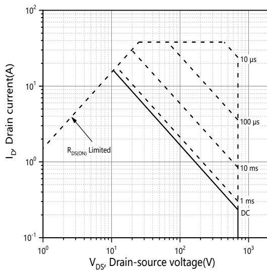
Figure 11. Safe operation area T_C=25^\circ C
