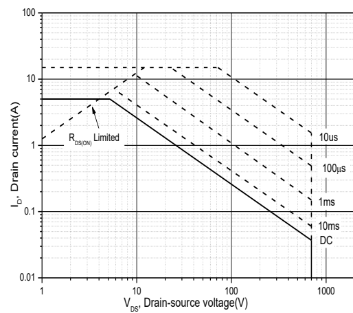
Figure 10. Safe operation area T_c = 25^{\circ}C
