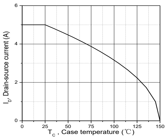
Figure 9. Drain current
