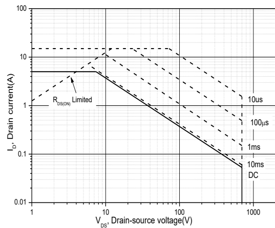
Figure 10. Safe operation area T_c = 25^{\circ}C
