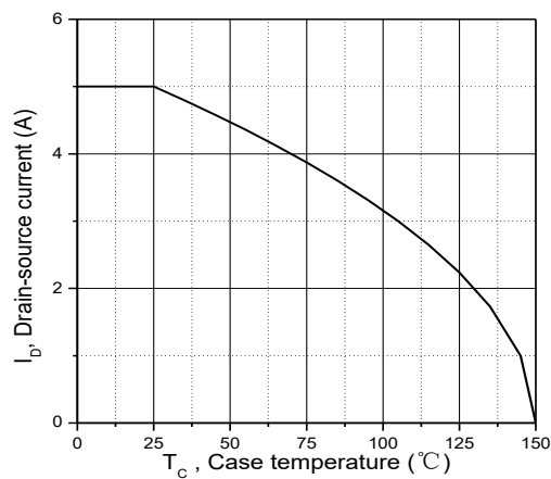
Figure 9. Drain current
