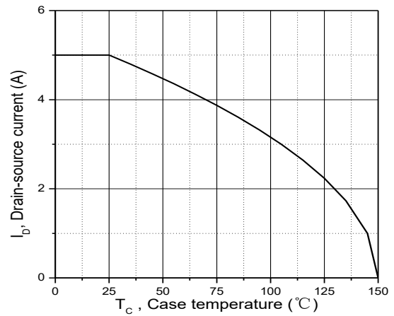
Figure 10. Drain current
