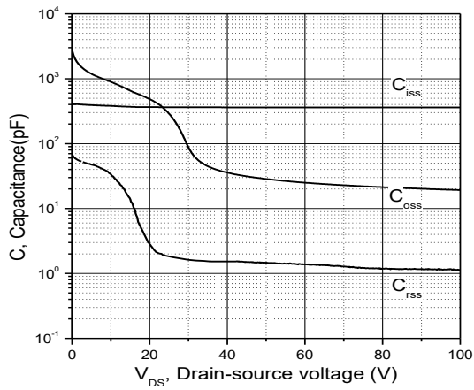
Figure 3. Typ. capacitances
