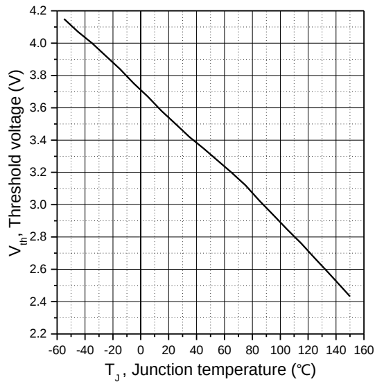
Figure 7. Threshold voltage
