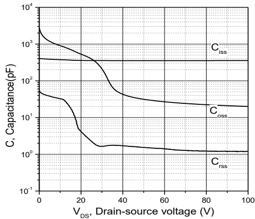
Figure 3. Typ. capacitances
