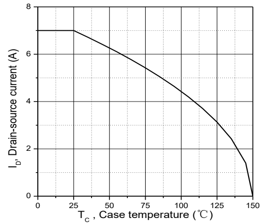
Figure 10. Drain current
