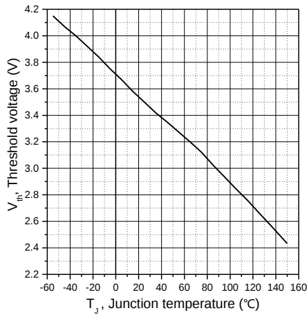
Figure 7. Threshold voltage
