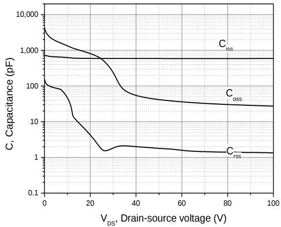
Figure 3. Typ. capacitances
