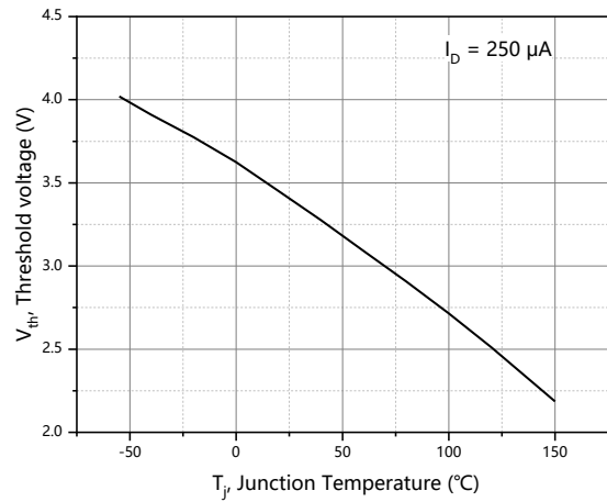
Figure 8. Threshold voltage
