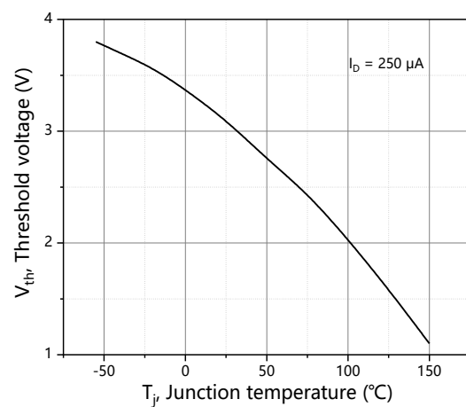
Figure 8. Threshold voltage
