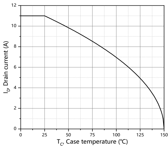
Figure 9. Drain current
