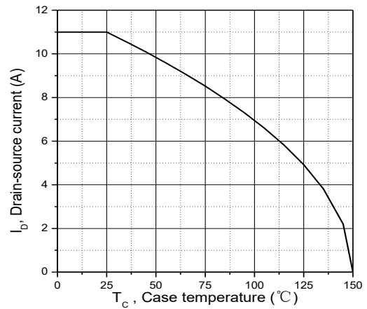
Figure 10. Drain current
