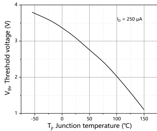
Figure 8. Threshold voltage
