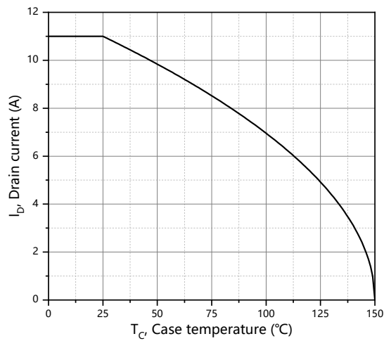
Figure 9. Drain current
