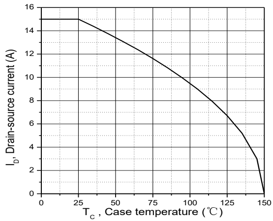
Figure 9. Drain current
