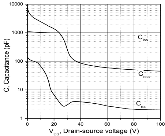
Figure 3. Typ. capacitances
