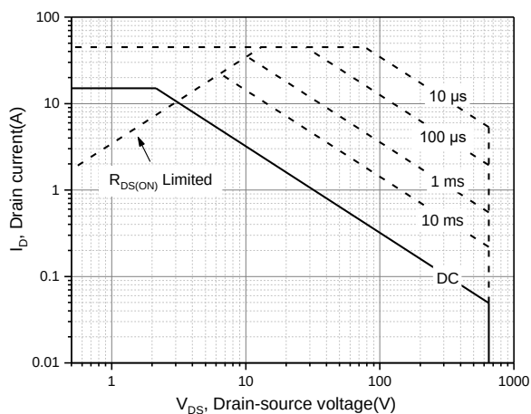
Figure 11. Safe operation area T_C=25\text{ °C}
