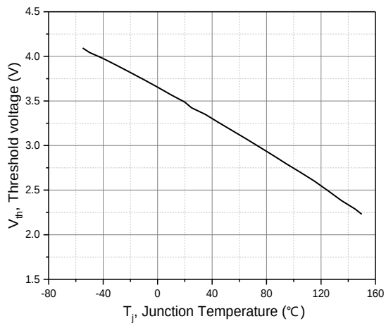
Figure 7. Threshold voltage
