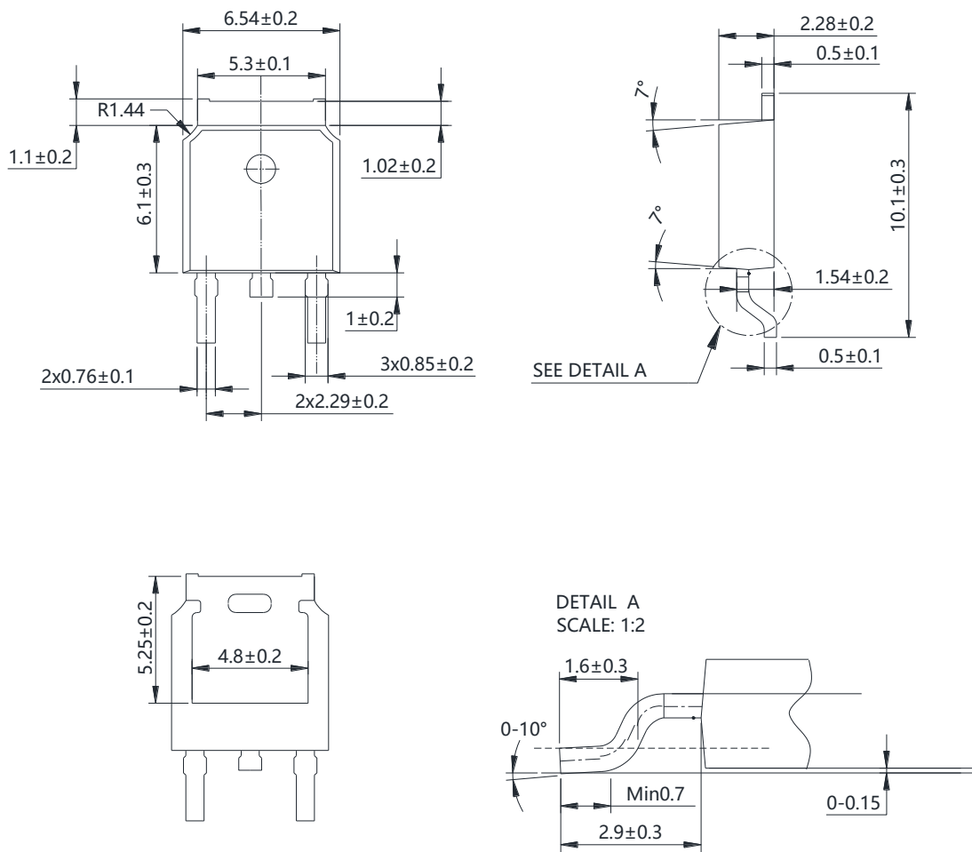
Version3: TO252-F package outline dimension
