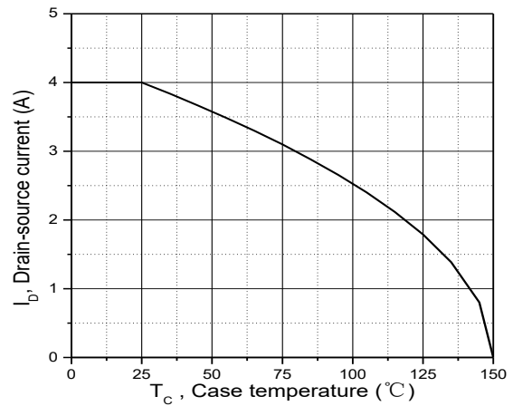
Figure 10. Drain current
