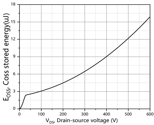
Figure 13. Typ. Coss stored energy
