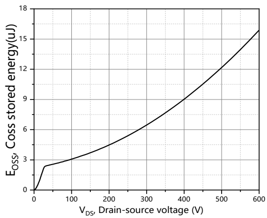
Figure 13. Typ. Coss stored energy
