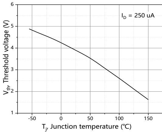
Figure 7. Threshold voltage
