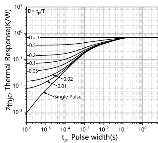
Figure 13. Max. transient thermal impedance
