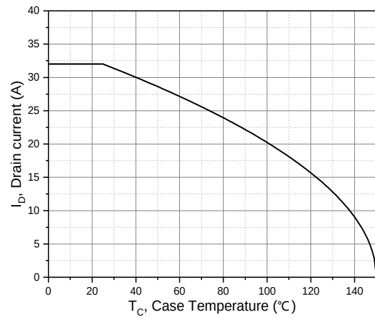
Figure 10. Drain current
