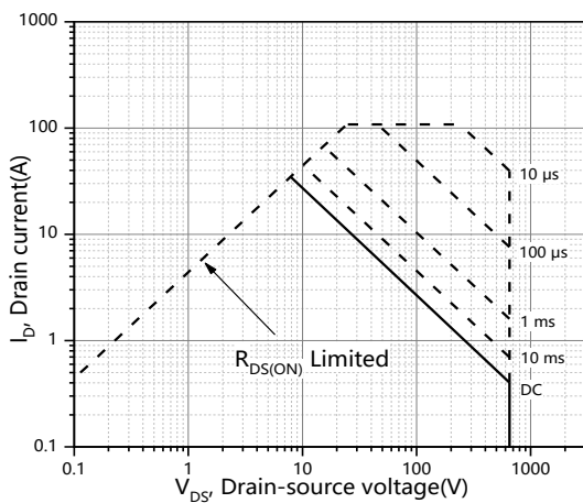
Figure 11. Safe operation area for T_C = 25 °C
