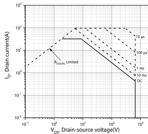
Figure 12. Safe operation area T_C=25^\circ\text{C}
