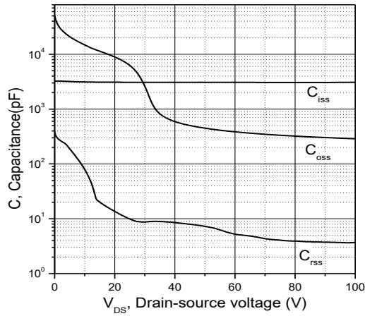
Figure 3. Typ. capacitances
