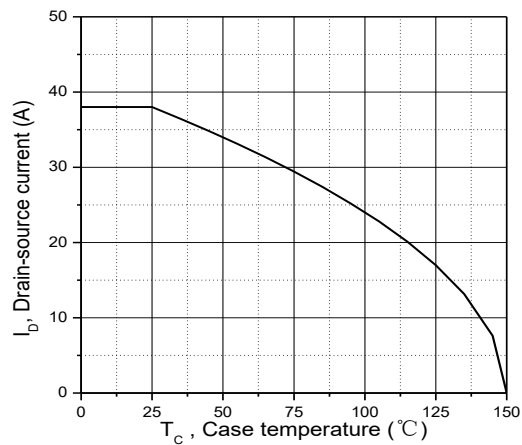
Figure 9. Drain current
