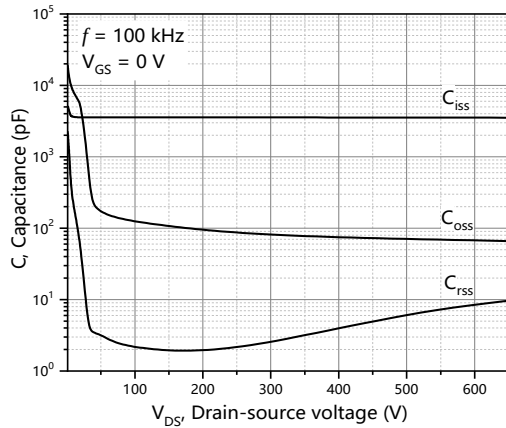
Figure 3. Typ. capacitances
