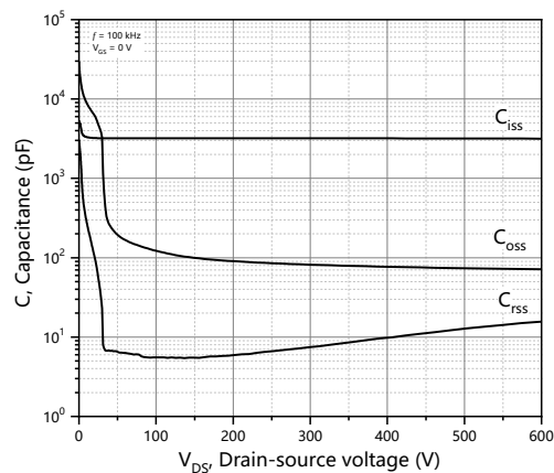
Figure 3. Typ. capacitances
