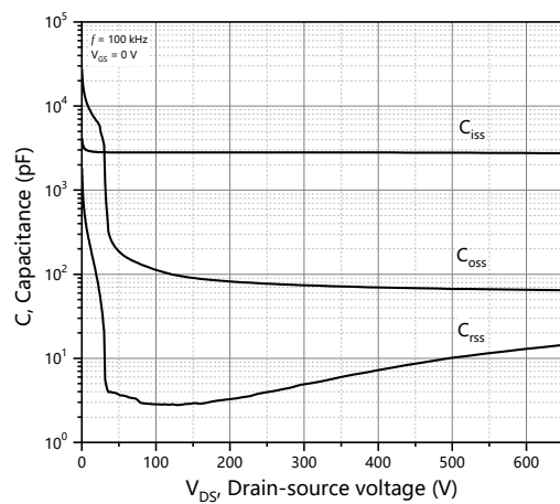
Figure 3. Typ. capacitances
