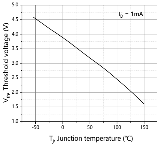
Figure 7. Threshold voltage
