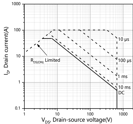
Figure 12. Safe operation area Tc=25°C
