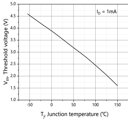
Figure 7. Threshold voltage
