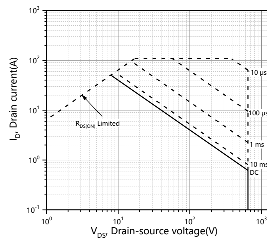
Figure 12. Safe operation area Tc=25°C
