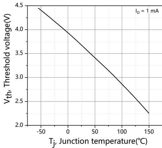
Figure 7. Threshold voltage
