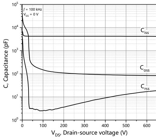
Figure 3. Typ. capacitances
