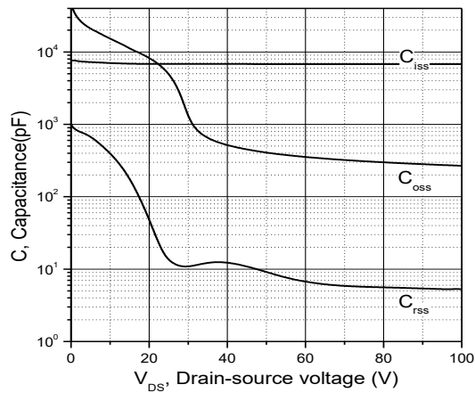
Figure 3. Typ. capacitances
