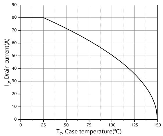
Figure 10. Drain current
