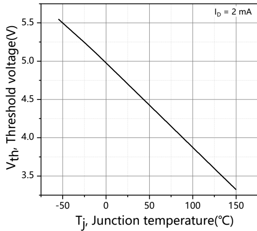
Figure 7. Threshold voltage
