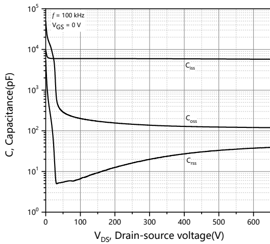
Figure 3. Typ. capacitances
