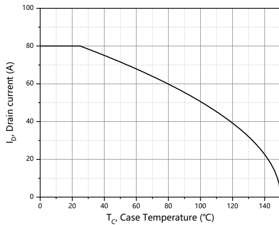
Figure 9. Drain current
