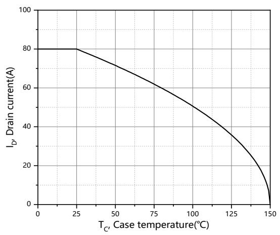
Figure 10. Drain current
