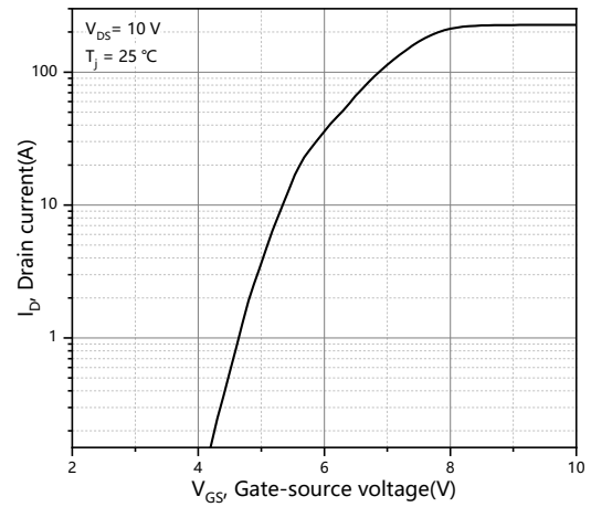
Figure 10. Drain current
