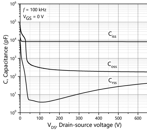
Figure 3. Typ. capacitances
