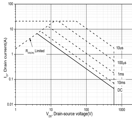
Figure 10. Safe operation area T_C=25\text{ }^{\circ}\text{C}
