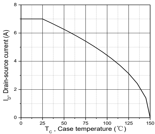
Figure 9. Drain current
