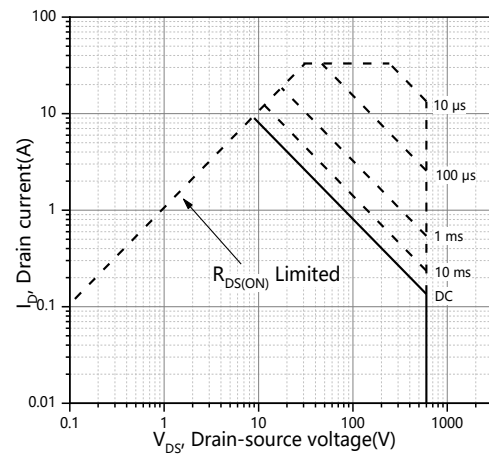
Figure 12. Safe operation area T_c=25^\circ C
