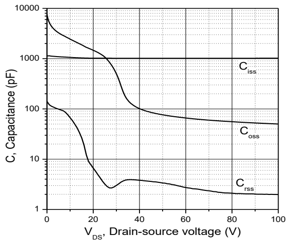
Figure 3. Typ. capacitances
