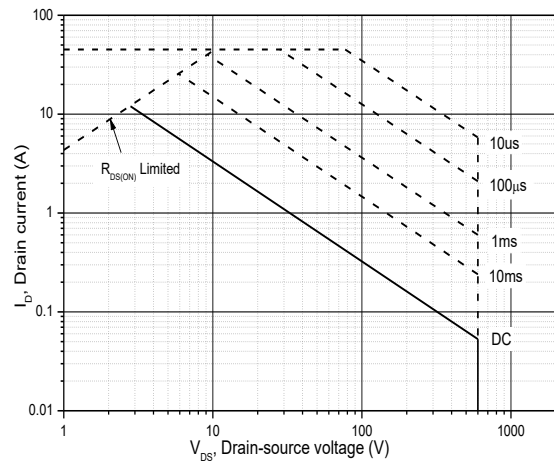
Figure 10. Safe operation area Tc=25 °C
