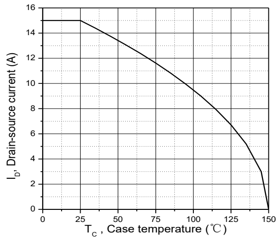
Figure 9. Drain current
