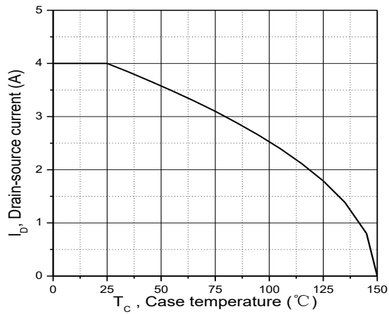
Figure 9. Drain current
